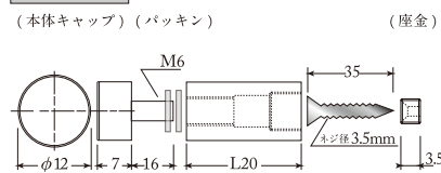
φ12×L20
