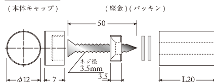
φ12×L20
